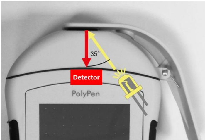
Fig. 2 Schema of reflectance measurement.
